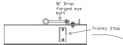
8:1 Scale View Cable anchor assembly and stop unit.
