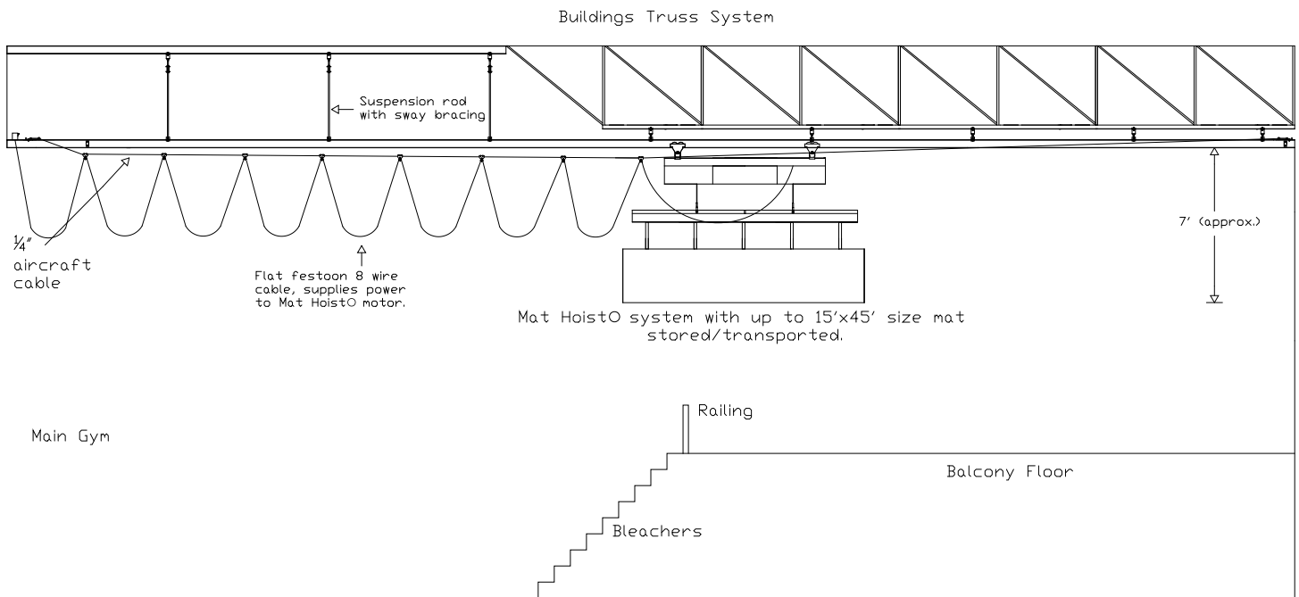
8:1 Scale View One ton maintenance free heavy duty trolley. Two trolleys required for end First travel
