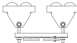
4:1 Scale view of double trolley system using CL-5 clamp. One double trolley each travel beam.
